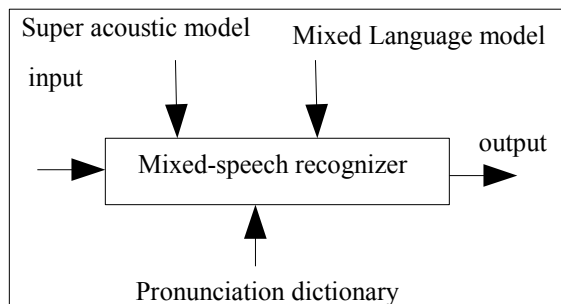
Figure 2. One-pass Framework
